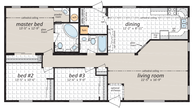
“The DE-363” 27' x 52' 1,404 sq.ft.
