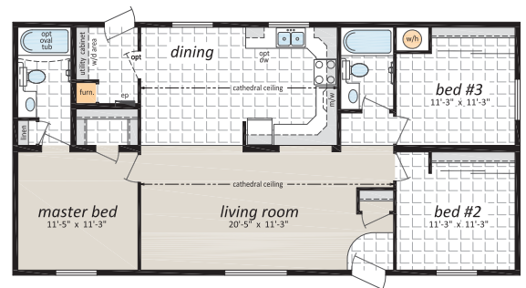
“The AM-862” 24' x 48' 1,152 sq.ft.
