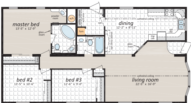
“The DE-362” 27' x 52' 1,404 sq.ft.
