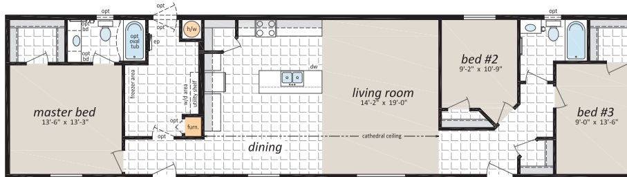
ML-205 20' x 76' • 1,520 sq. ft.
