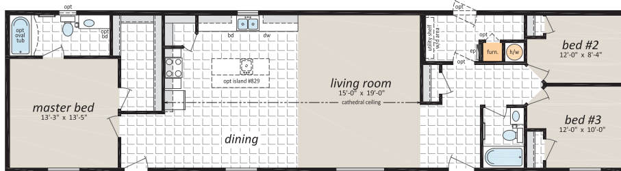
ML-204 20' x 76' • 1,520 sq. ft.
