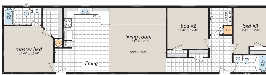
ML-202 20' x 76' • 1,520 sq. ft.
