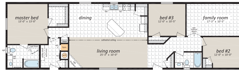
ML-6 22' x 76' • 1,672 sq. ft.
